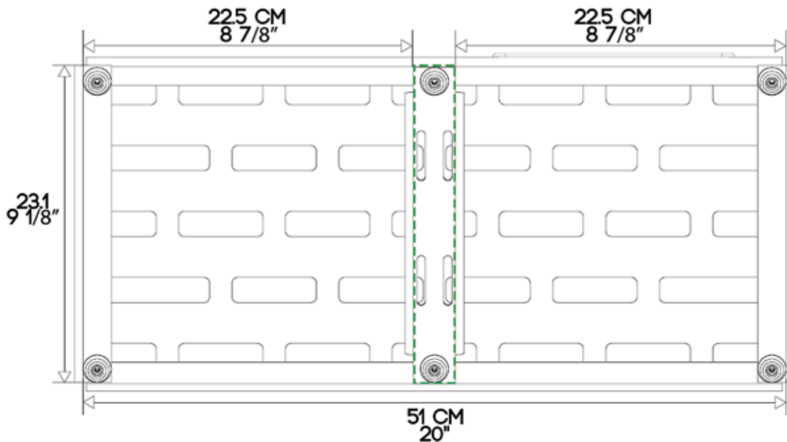
UNDERSIDE VIEW
