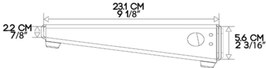
SIDE VIEW
