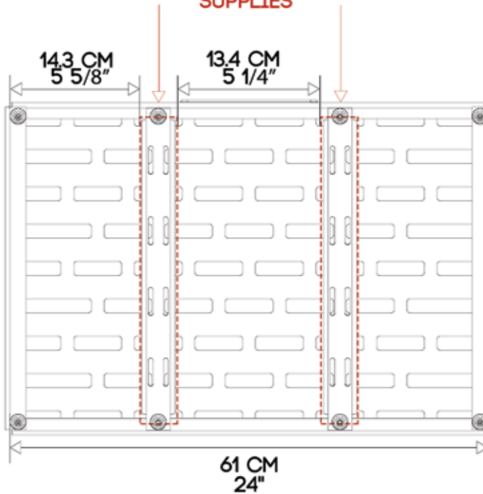
UNDERSIDE VIEW
